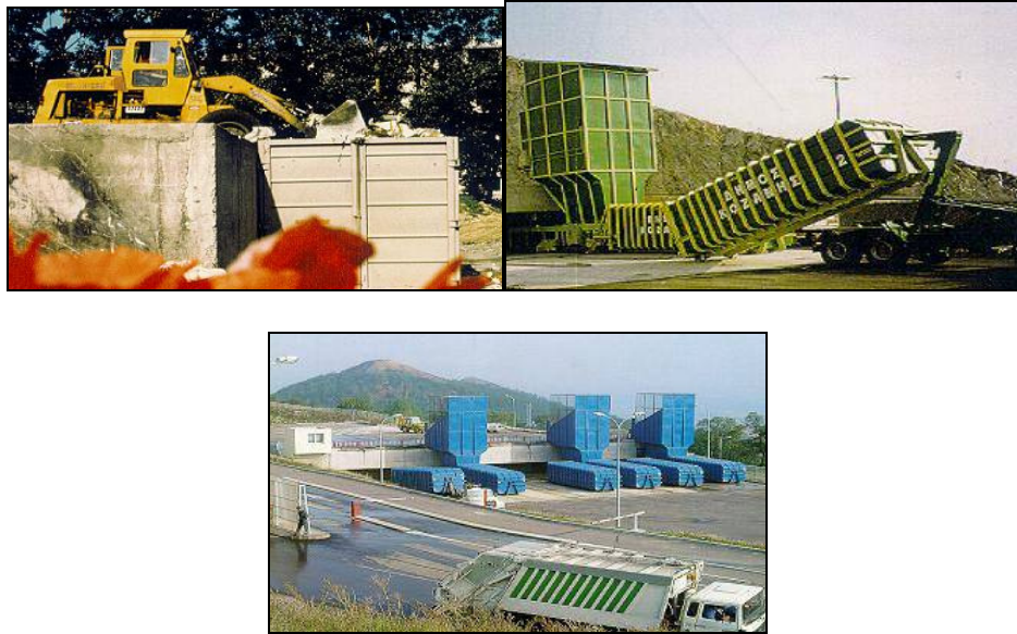
Figure 3-54: Waste disposal in container with no compaction, hopper compaction and automated transfer station
