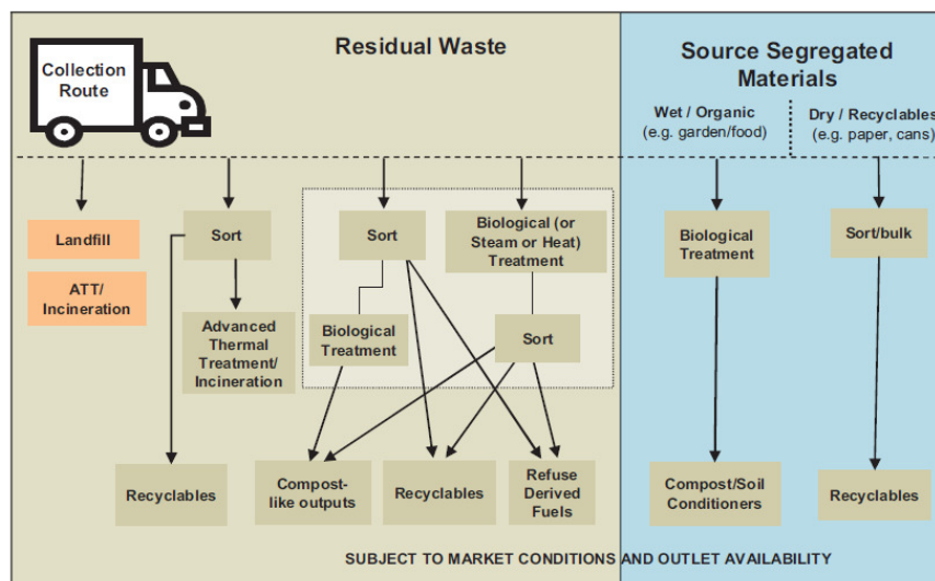
Figure 3-103: Options for Recovery & Treatment of Municipal Solid Waste (DEFRA 2007)
