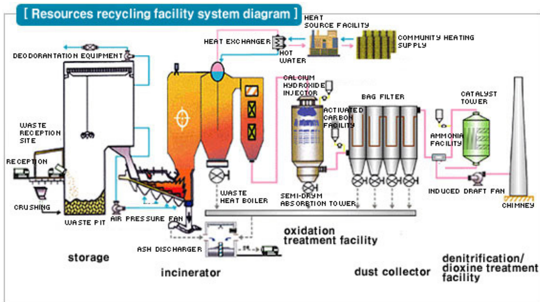
Figure 3-90: Typical layout of incineration plant
