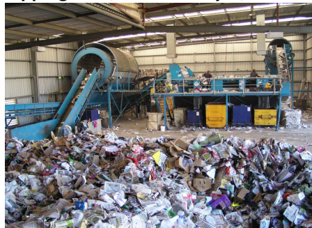
Figure 3-65: Tripping area, feed conveyer, trammel, picking line
