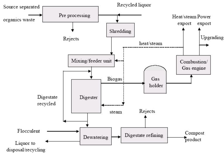
Figure 3-82: Anaerobic digestion process
