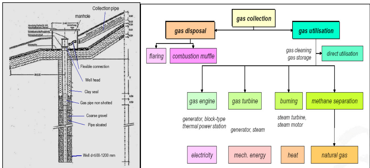
Figure 3-102: (a) Biogas collection and (b) Biogas utilization
