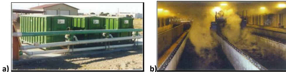
Figure 3-76: a) Composting Beds, b) Rotating drum system
