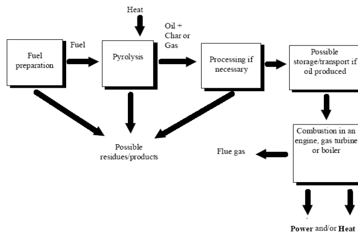
Figure 3-92: Schematic representation of pyrolysis process
