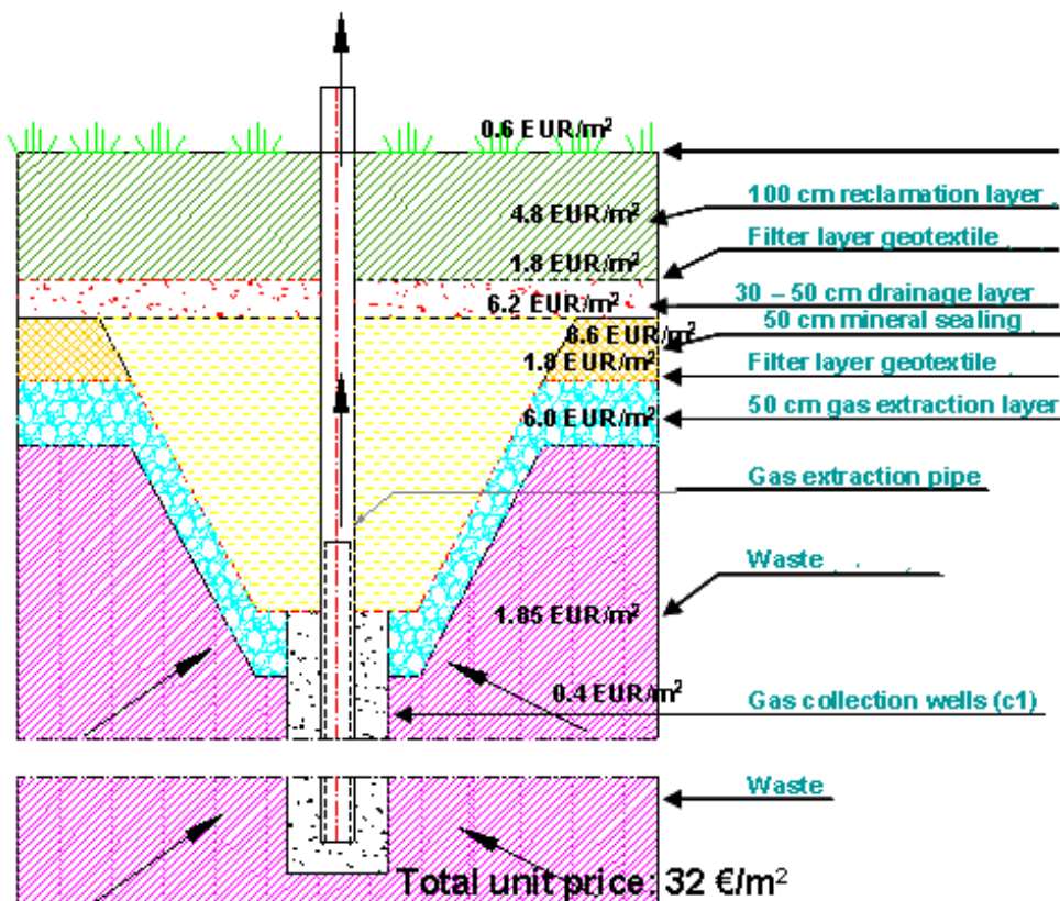
Figure 3-105: Section of remediated landfill after model "C1" (100,000 – 500,000 m 3 )
