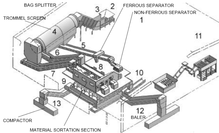
Figure 3-59: Typical layout of MRF plant
