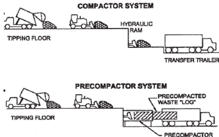
Figure 3-53: Compaction System in a transfer station
