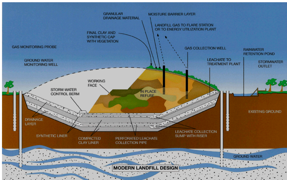
Figure 3-96: Illustration of a landfill setup
