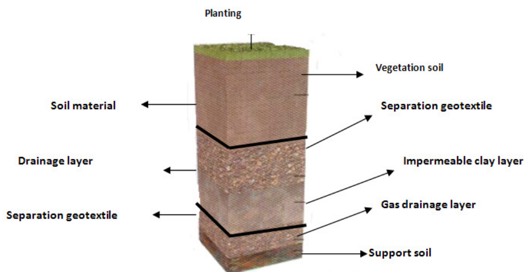
Figure 3-94: Construction of top cover layers
