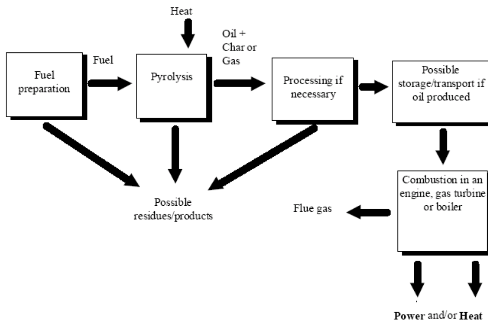
Figure 3-91: Gasification
