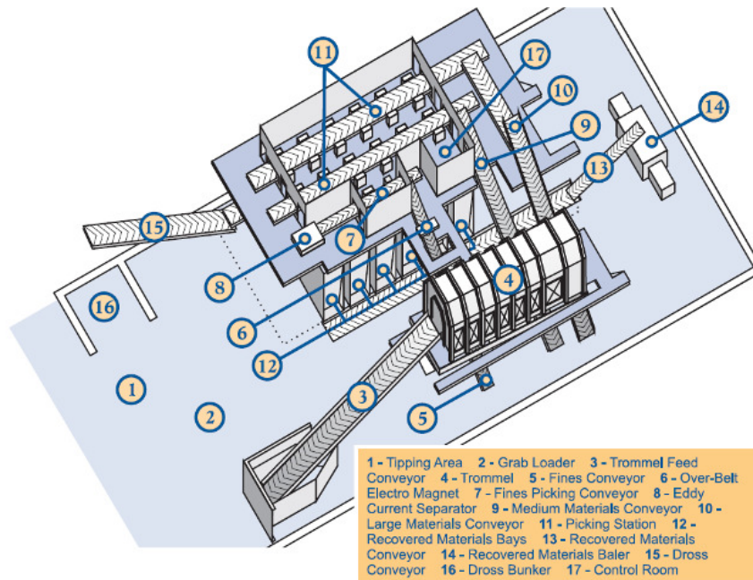
Figure 3-58: Typical layout of MRF plant
