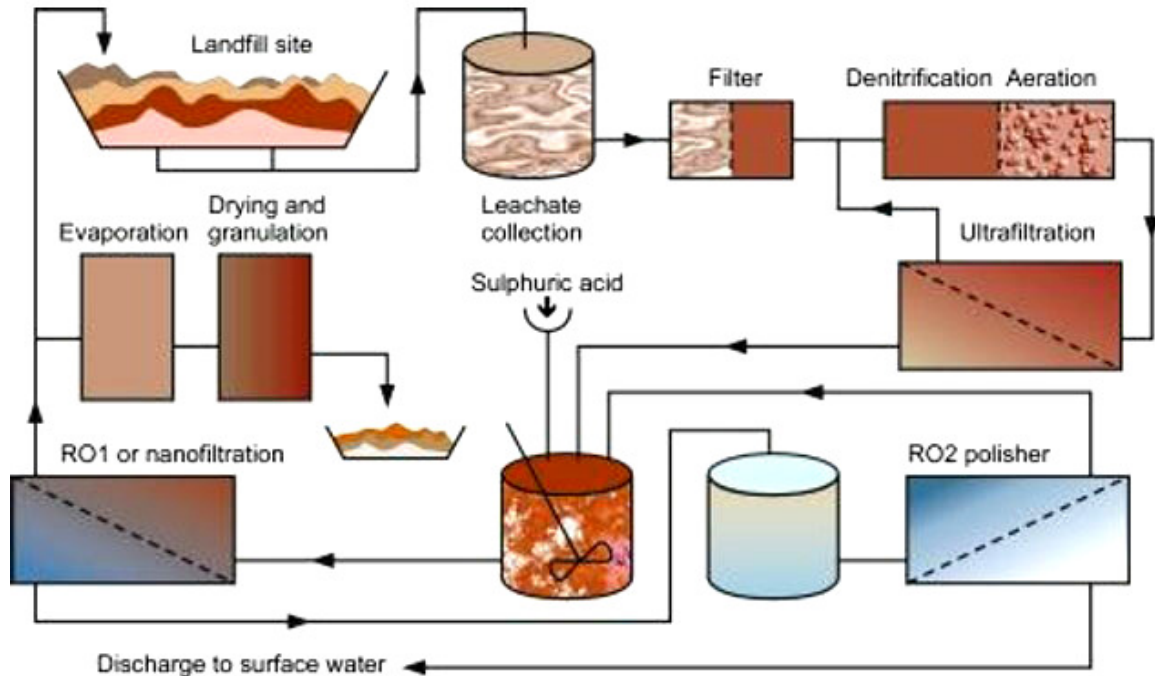
Figure 3-101: Leachate treatment
