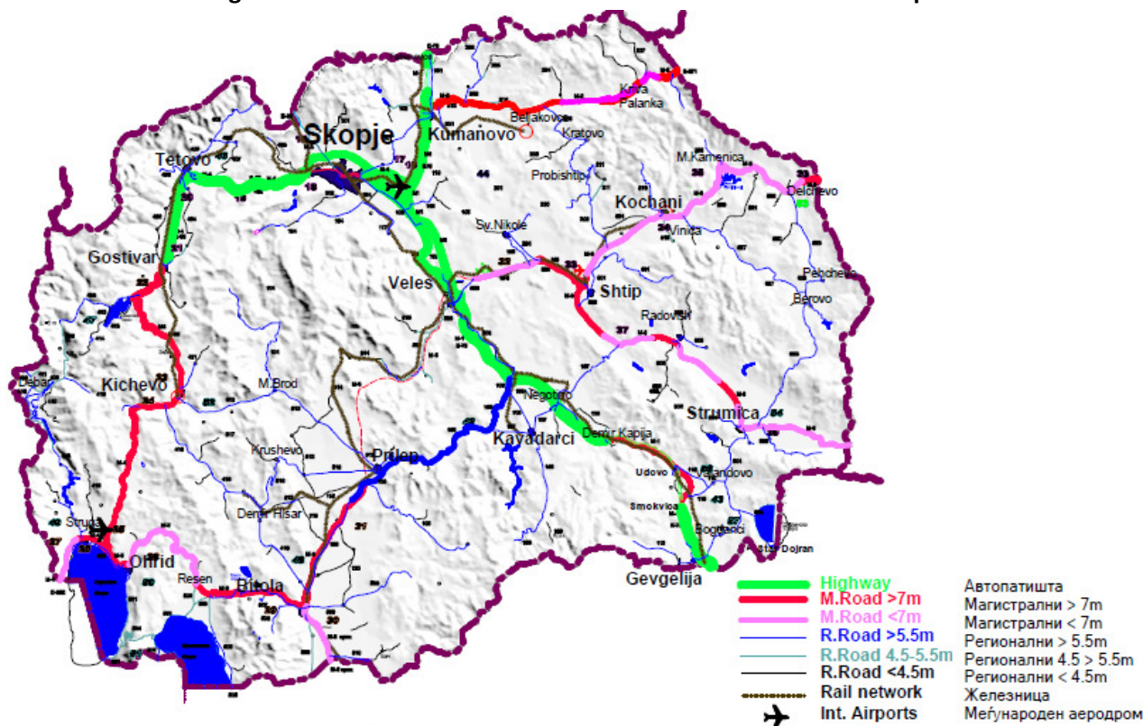
Figure 2-19: Road network in relation with other modes of transport
