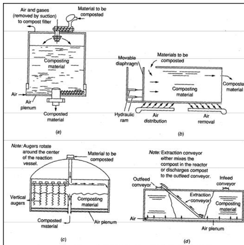
Figure 3-77: Basic closed composting systems (A&C: vertical reactors, B&D: horizontal reactors)
