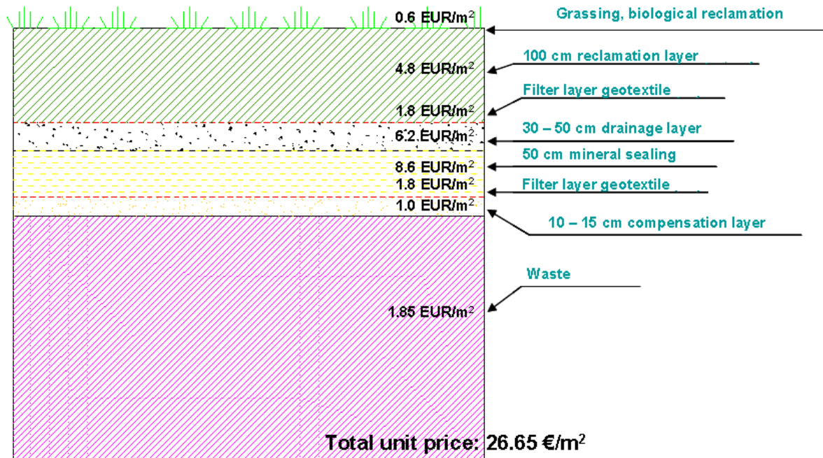
Figure 3-104: Section of remediated landfill after model "B"
