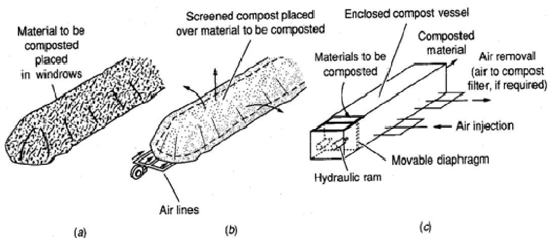
Figure 3-70: Simplified illustration of the 3 basic composting systems: (a) agitated windrows, (b) aerated static piles, (c) closed systems
