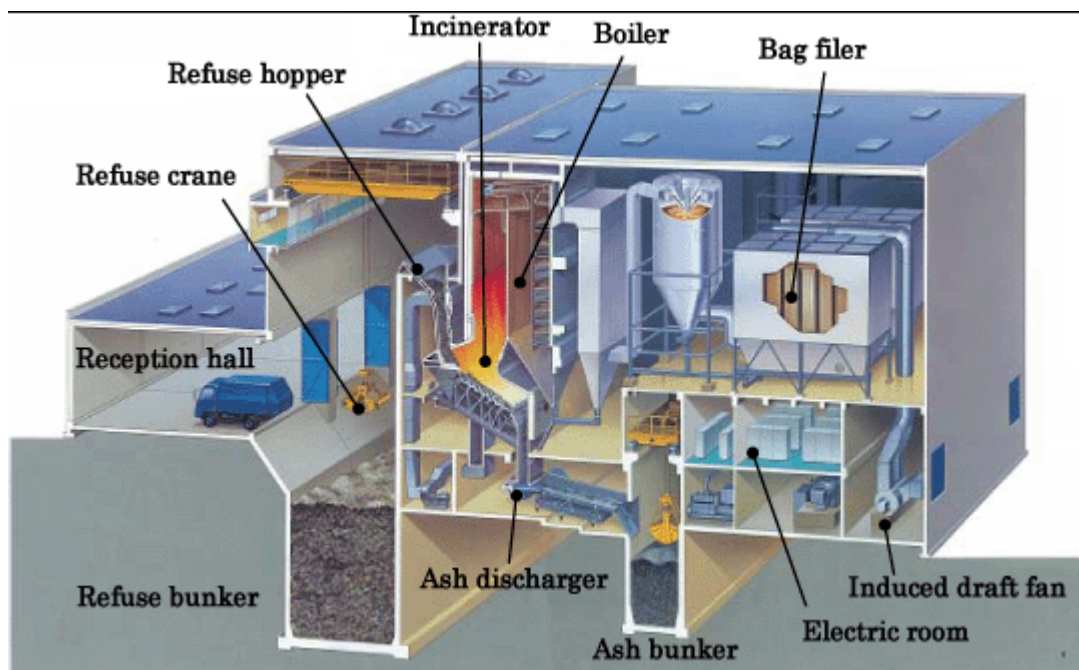
Figure 3-89: Intersection of typical layout of incineration plant
